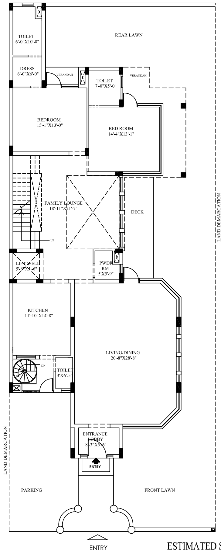
GROUND FLOOR PLAN Total = 2359.12 Sq. ft.
