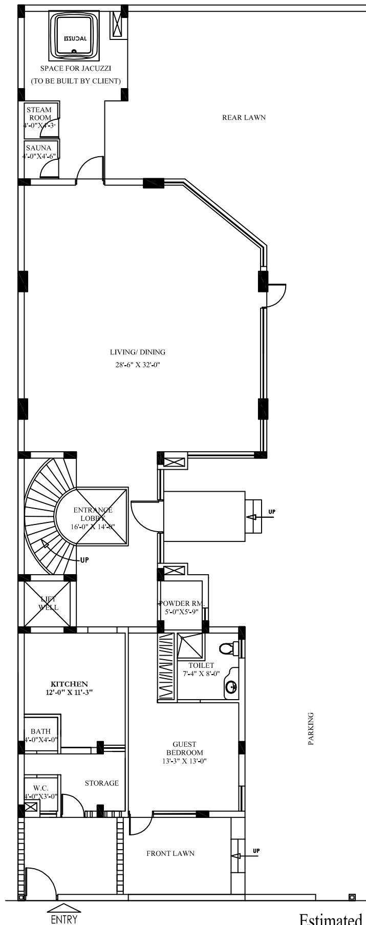
GROUND FLOOR PLAN Total = 2221.88 Sqft
